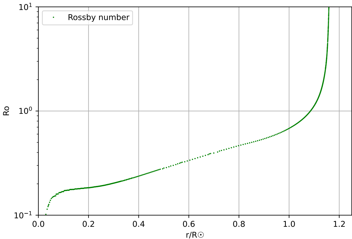
Rossby number, profile 164, age 8.58 \times 10^9
